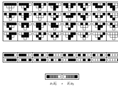
rule 90
