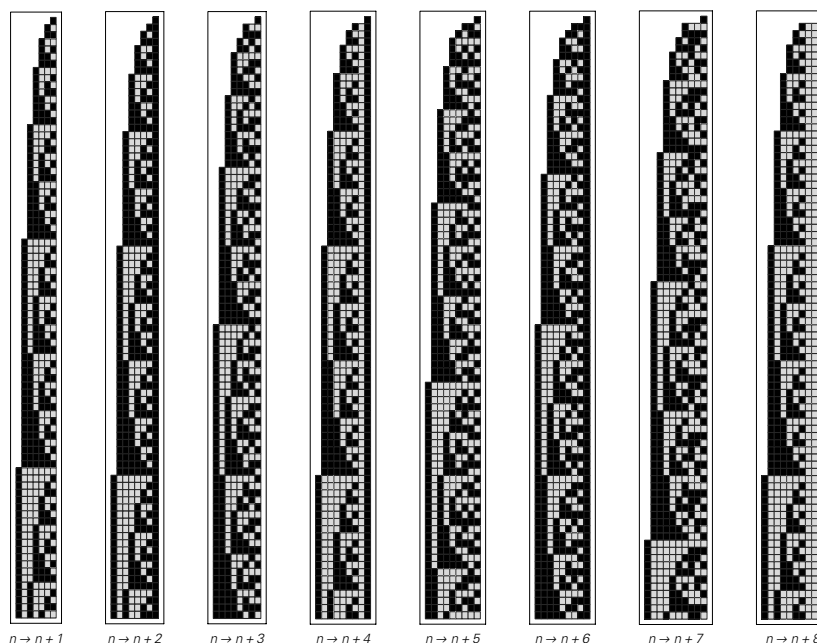
Digit sequences in base 2 of numbers obtained by starting with 1 and then successively adding a constant at each step. All these patterns ultimately have the same overall nested form.
