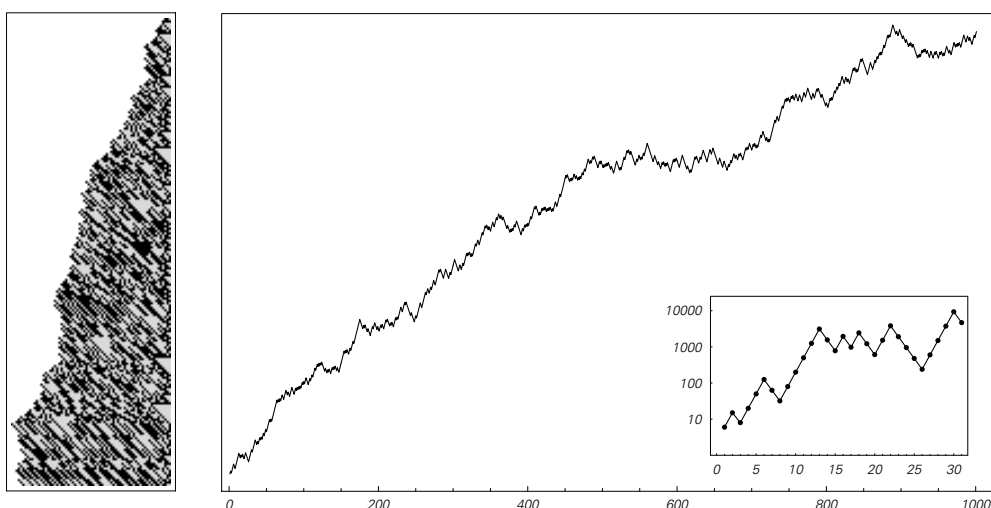
The results of following the same rule as on the previous page, starting from the value 6. Plotted on the right are the overall sizes of the numbers obtained for the first thousand steps. The plot is on a logarithmic scale, so the height of each point is essentially the length of the digit sequence for the number that it represents—or the width of the row on the left.
