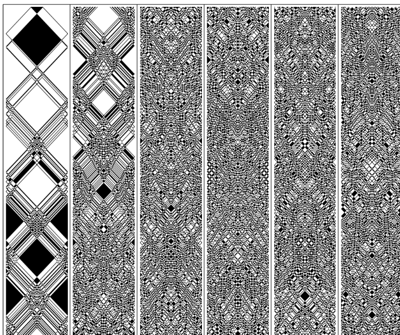
A reversible cellular automaton that exhibits seemingly irreversible behavior. Starting from an initial condition in which all black cells or particles lie at the center of a box, the distribution becomes progressively more random. Such behavior appears to be the central phenomenon responsible for the Second Law of Thermodynamics. The specific cellular automaton used here is rule 122R. The system is restricted to a region of size 100 cells.
